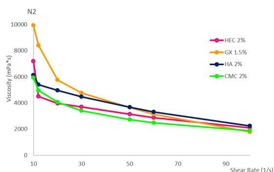
Fig. 2. Rheological behavior of NADES-hydrogels with NADES solvent N2
