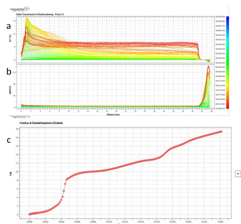
Fig. 1. Examples of Turbiscan profiles showing changes in the (a) transmission, (b) backscattering and (c) TSI over 24 hours.
