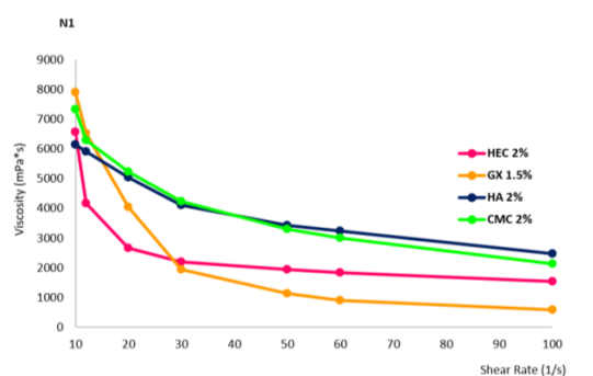
Fig. 1. Rheological behavior of NADES-hydrogels with NADES solvent N1
